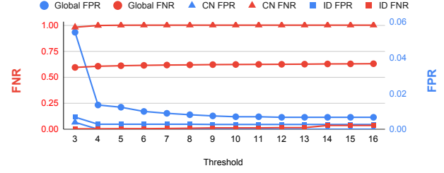
Figure 4: The Efficacy of the AS threshold heuristic— Generated by comparing statistical AS thresholding to the results of certificate validation and blockpage matching on the global scale, China and Indonesia, respectively.
